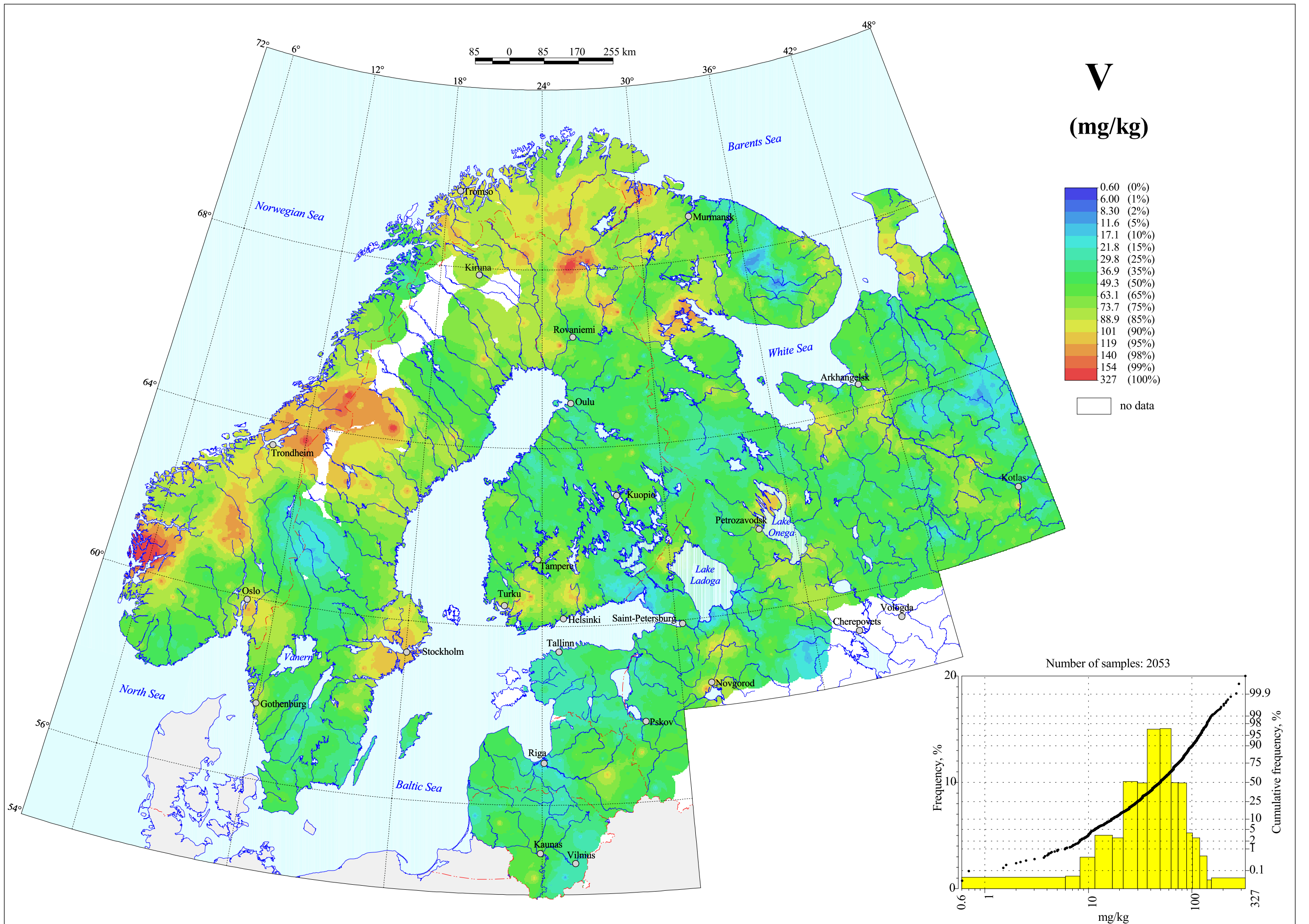
Vanadium in C-horizon, Grain Size <2 mm, Total Content
